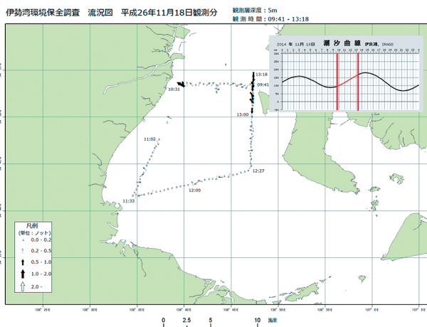
Fig. 16. Result of current observation in November 18, 2014.
