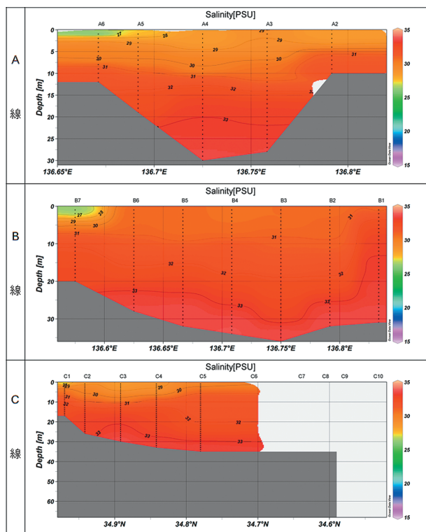
Fig. 49. Result of salinity observation in March, 2015.
