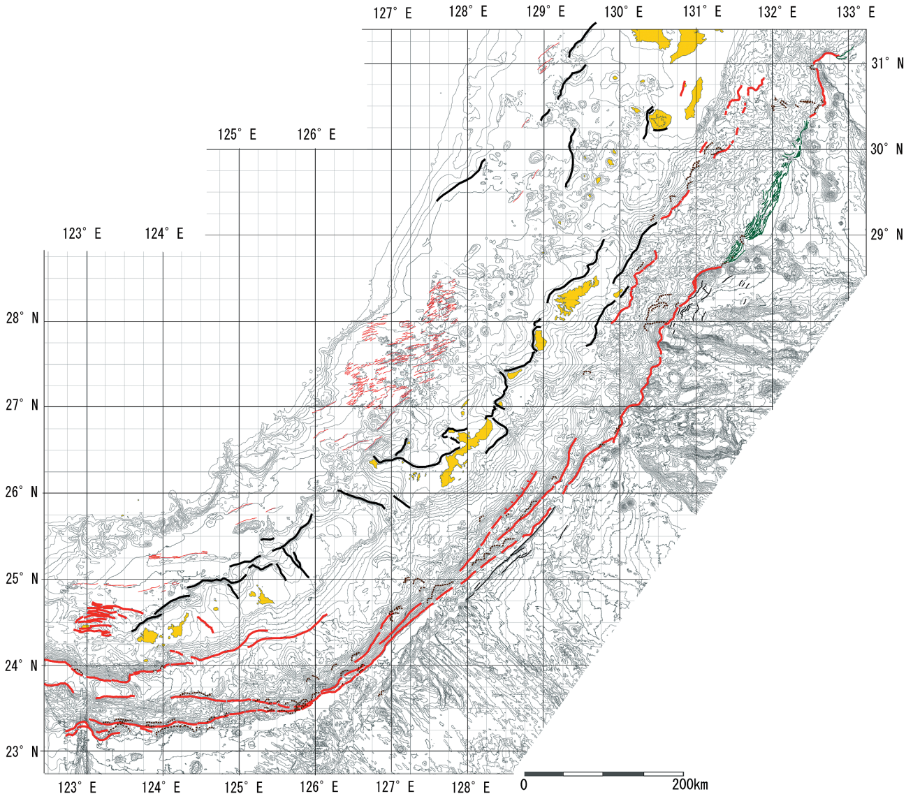
Fig. 10. Map showing active faults, volcanoes, landslides along Nansei-Shoto Trench (thick red line: active fault, red arrow: warping, thick black line : presumed active fault, thin blue line: presumed strike-slip fault, thin green line: active fault in young accretion prism, thin red line: active fault in Okinawa Trough, thin blue line: presumed strike-slip fault, thin black line: normal fault on outer rise), landslide (dashed brown line) superimposed on bathymetry (contours in 200 m).
